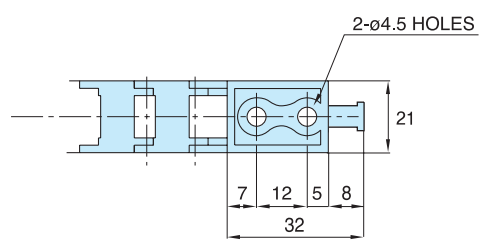
Fixed Bracket
