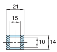
A-A Cross Section
