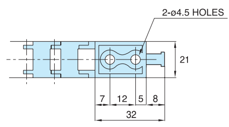
Moving Bracket
