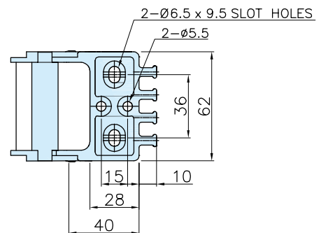
Moving Bracket
