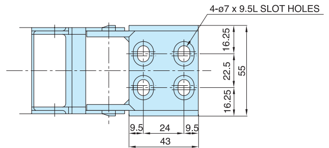
Moving Bracket
