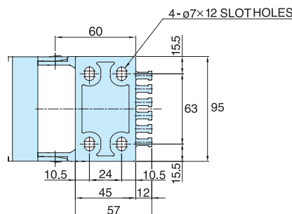
Moving Bracket
