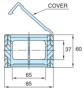
A-A Cross Section
